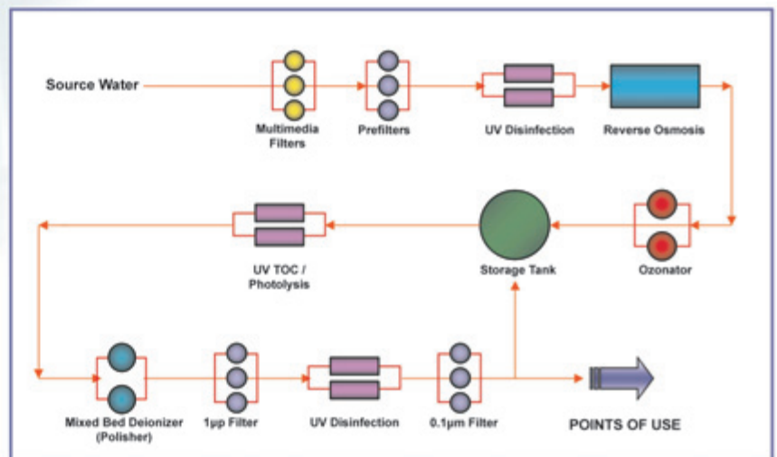
The role of UV in Ultrapure Water Production
